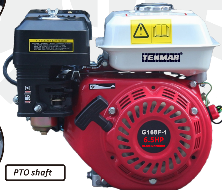
OHV Structure Compact and light weight
